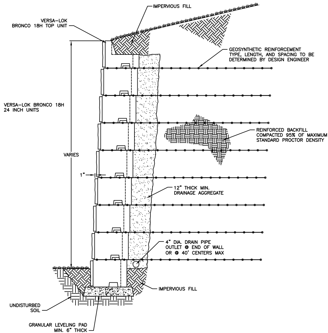
BRONCO 18H REINFORCED RETAINING WALL 24 INCH UNITS SCALE: NONE
